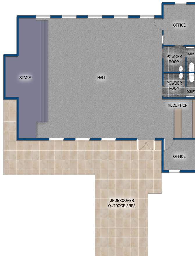
FLOOR PLAN
